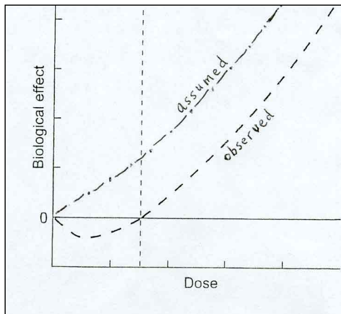
Fig.9. Dose and effect relationship with regard to radiation hazard. Very conservative assumptions have been made in setting guidelines.
