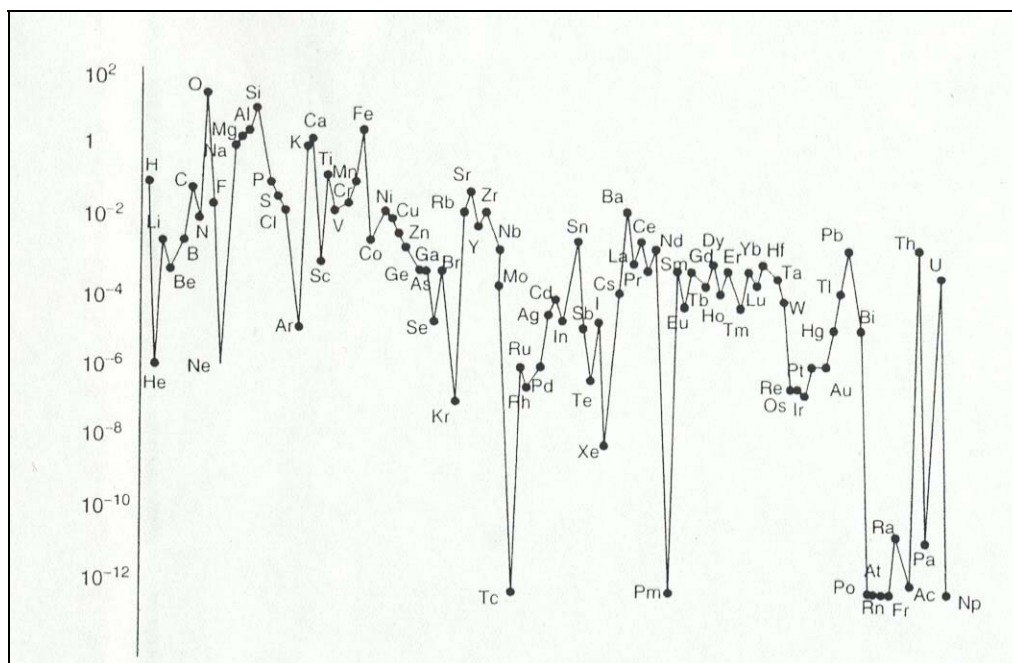
Fig. 2. Average concentration (in wt.%) of elements in the Earth's crust 1 .
