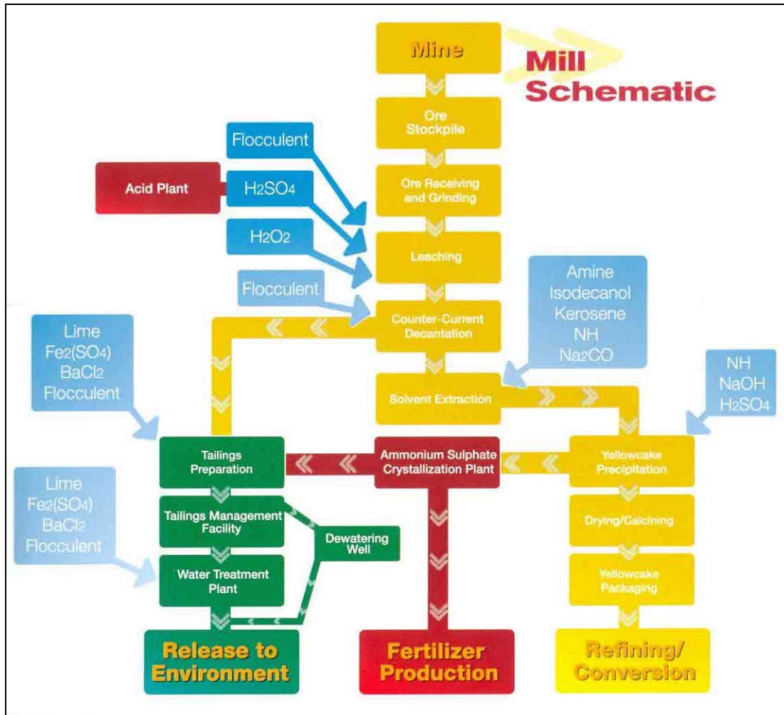
Fig. 5. Mill Schematic at McClean Lake, Saskatchewan. (Source: AREVA Resources Canada Inc.)
