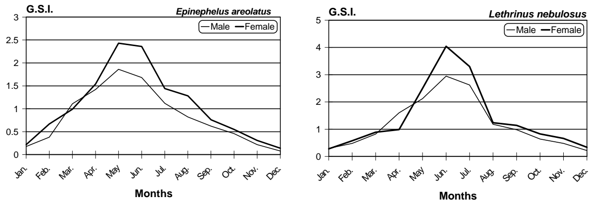
Fig. 2: Gonadosomatic index of E. areolatus and L. nebulosus in Halaieb/Shalatieh area Red Sea
