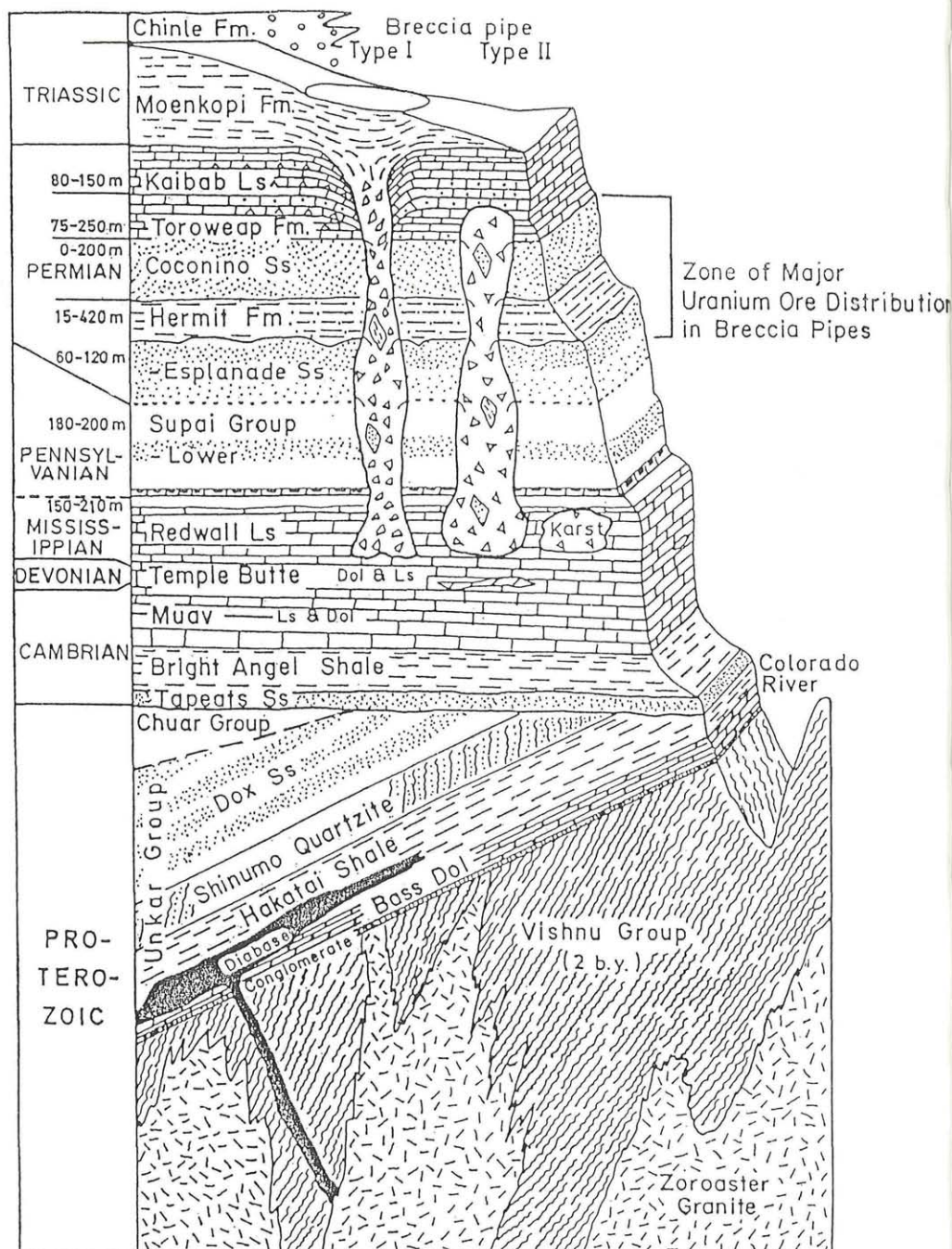
Figure 2: Schematic stratigraphic section of the Grand Canyon region showing position and mode of collapse breccia pipes (type I outcropping, type II blind). (Modified after drawing by HOLLAND, R. F., unpubl.; stratigraphy based on BREED & ROAT 1976.)
