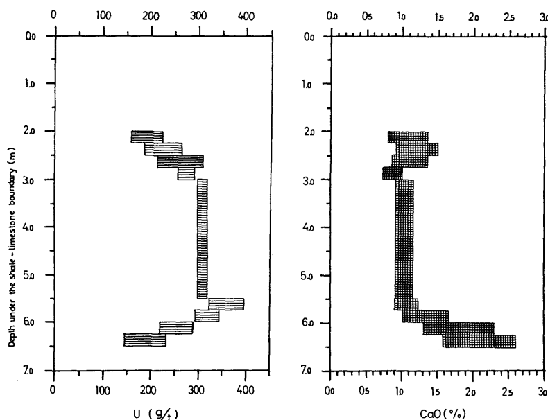
FIG. 7. Average content of uranium and lime in the shale (95% confidence limits based on a set of 20 drill cores).
