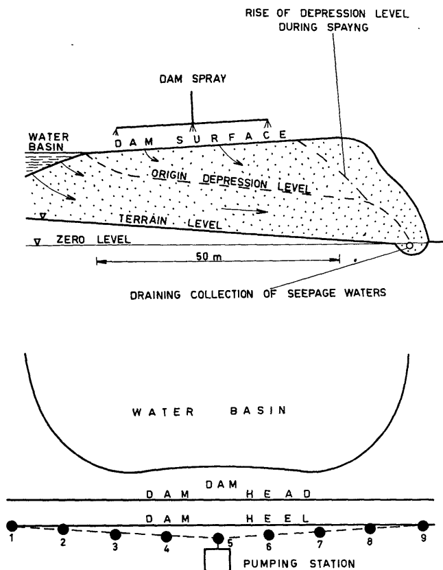
FIG. 1. Diagram of seepage and water withdrawal from the tailings pond: 1, 2 etc. individual shafts for seepage water.
