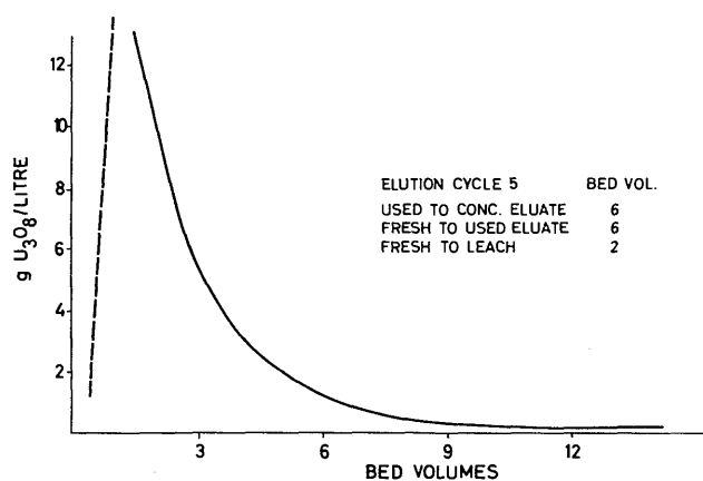
FIG. 5. Elution curve - set 6.
