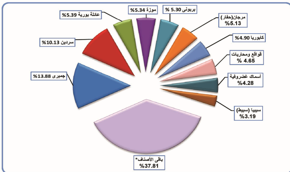
Figure 3-1-2 Qualitative structure (%) of the most important species of Med. Sea-2011
