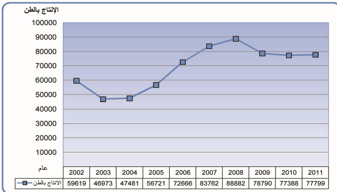
Figure 3-1-1 Catch trend of Mediterranean Sea / MT, 2002 - 2011
