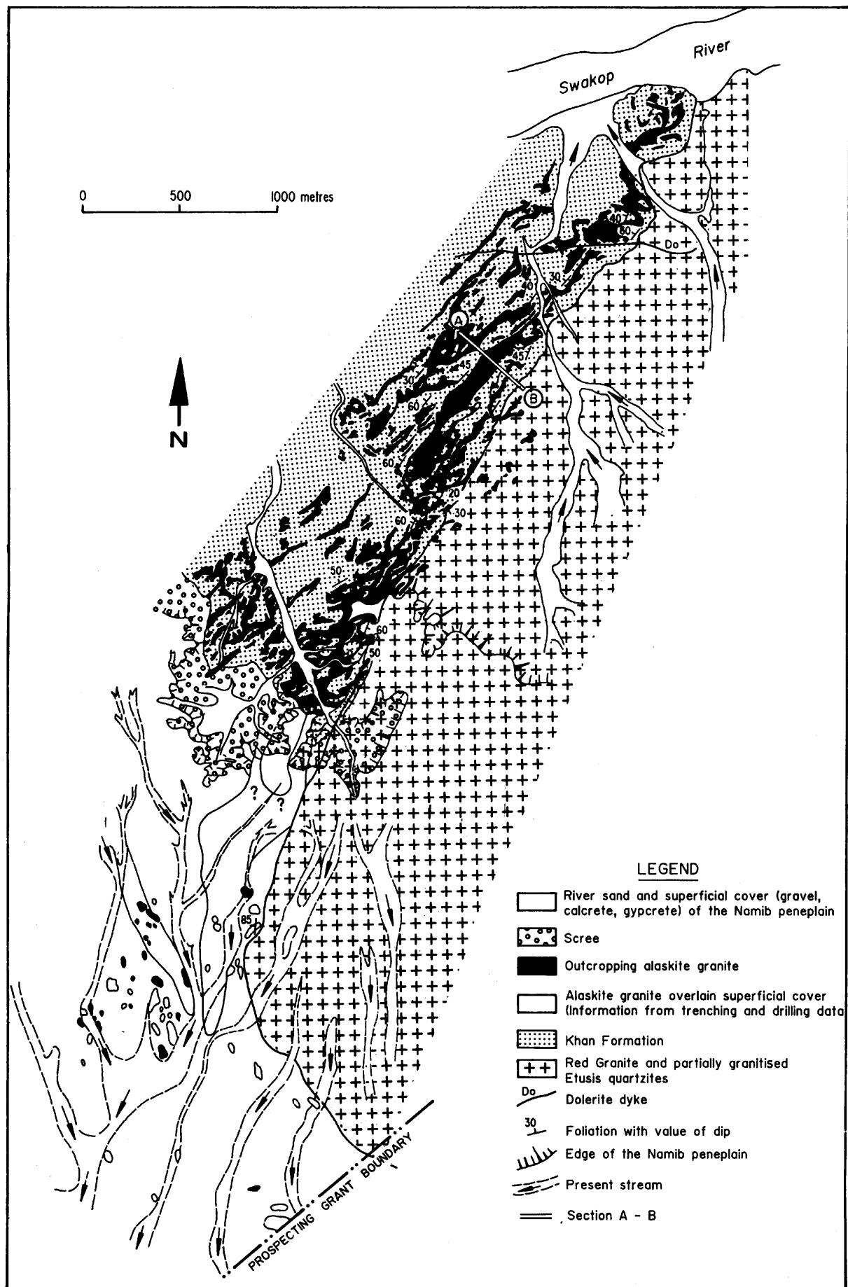
Figure 11: Generalised geology of the Goanikontes deposit showing the distribution of the alaskite (after Mouillac et al., 1986).
