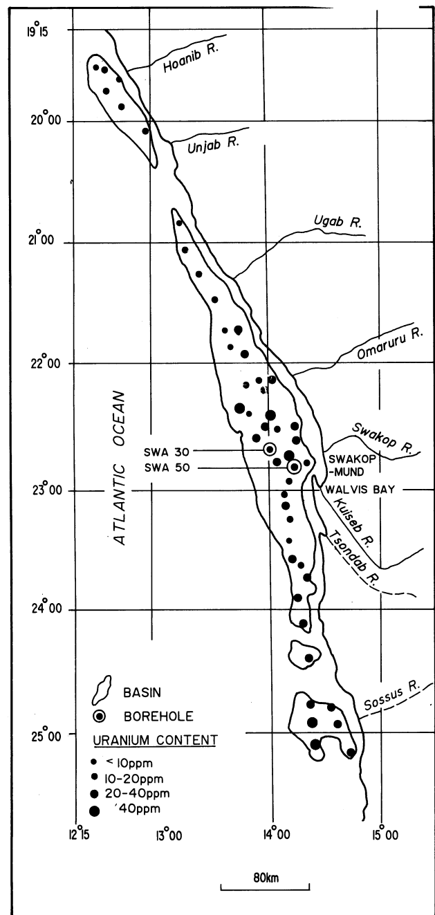
Figure 22: Offshore uranium occurrences (after Hambleton-Jones, 1983).
