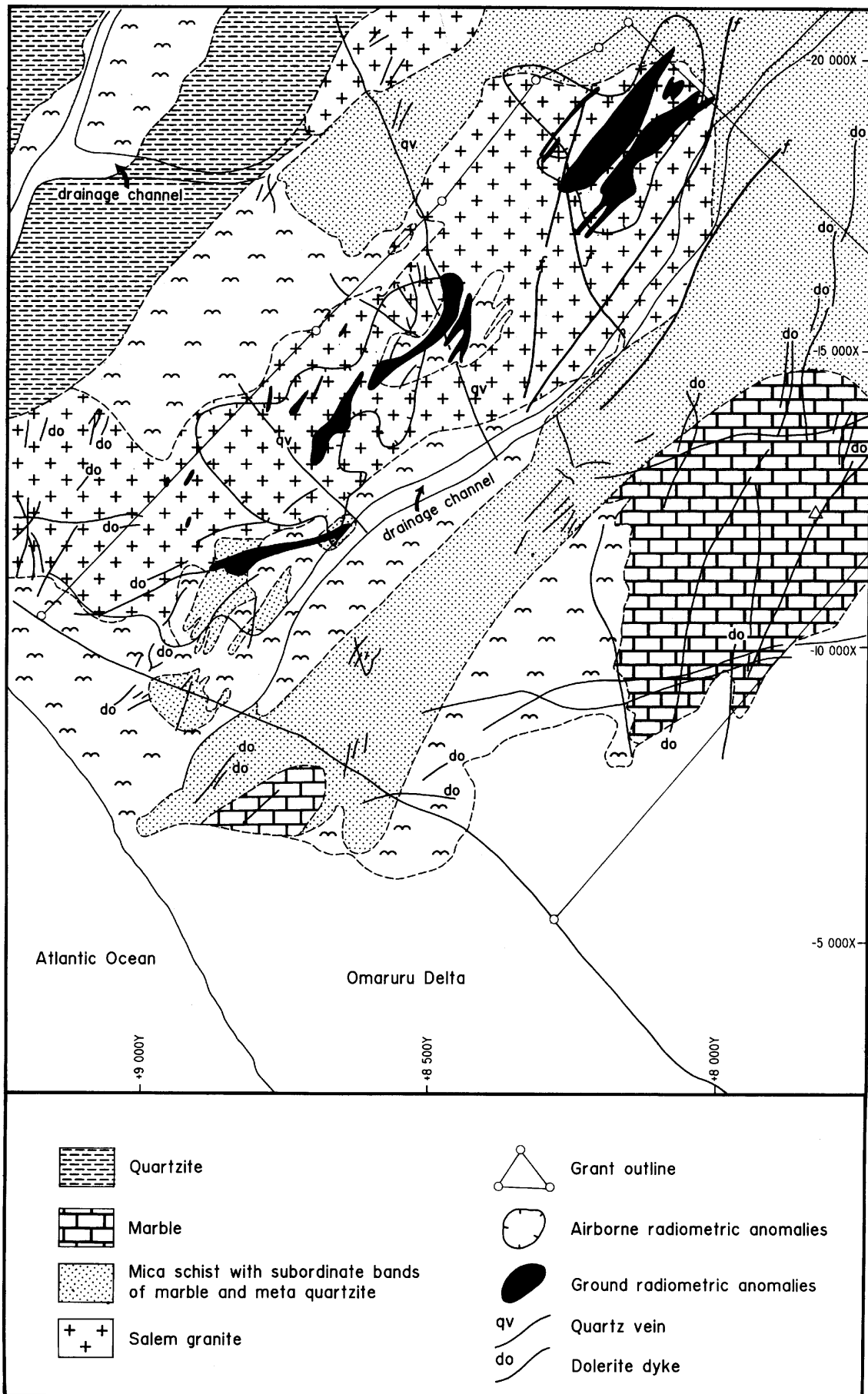
Figure 17: General geology of the Mile 72 area (after General Mining and Finance Corporation).
