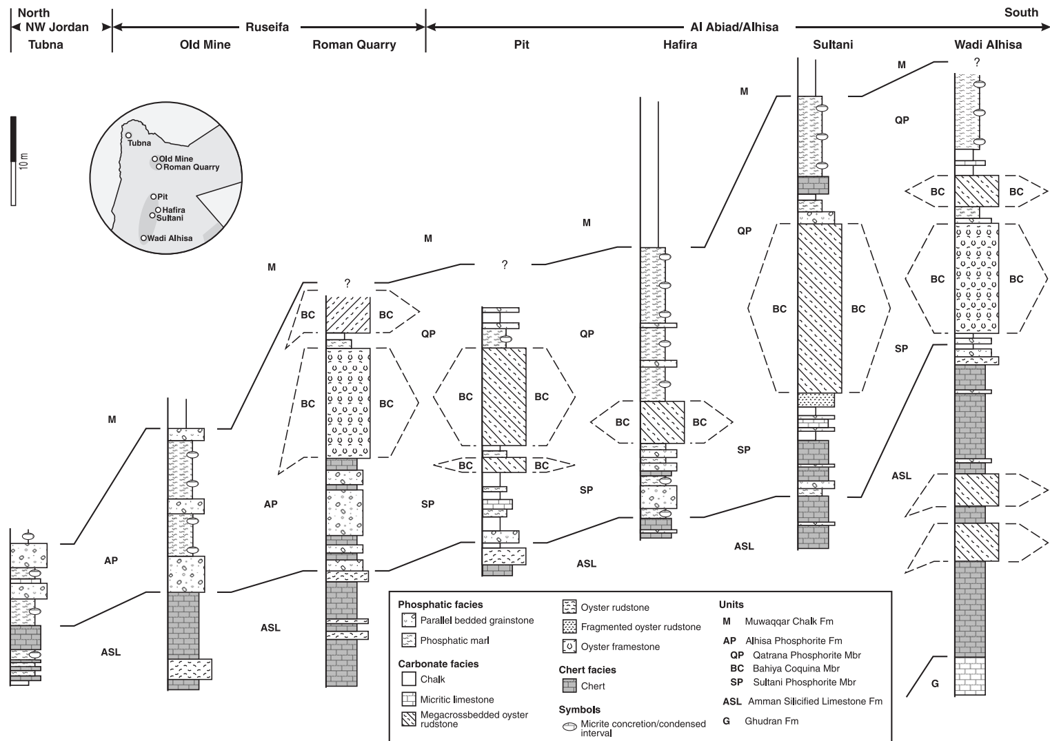
Fig. 6. Generalized fence diagram showing the regional stratigraphic framework of the Alhisa Phosphorite Formation. Sections from Tubna, Hafira, Sultani, and Wadi Alhisa have been compiled from Sadaqah (2000). Inset shows the location of the sections used to construct the fence diagram. The section is hung on the top of the Amman Silicified Limestone Formation.
