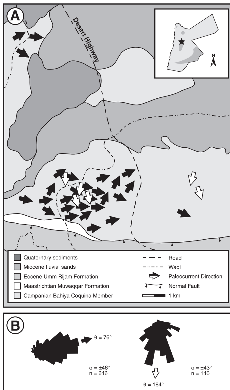
Fig. 5. Geological map with mean paleocurrent directions for the Bahiya Coquina member of the Alhisa Phosphorite Formation. Black arrows record east- and northeast-directed flow. White arrows indicate south-directed flow.
