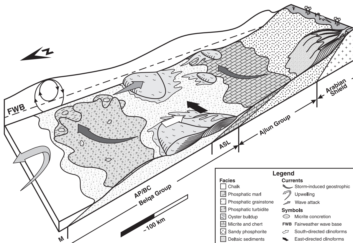
Fig. 7. Paleogeography and current regime during the deposition of the Belqa Group. Refer to text for discussion. The reconstruction of nearshore environments is based on Glenn and Arthur (1990) and Abed and Amireh (1999).
