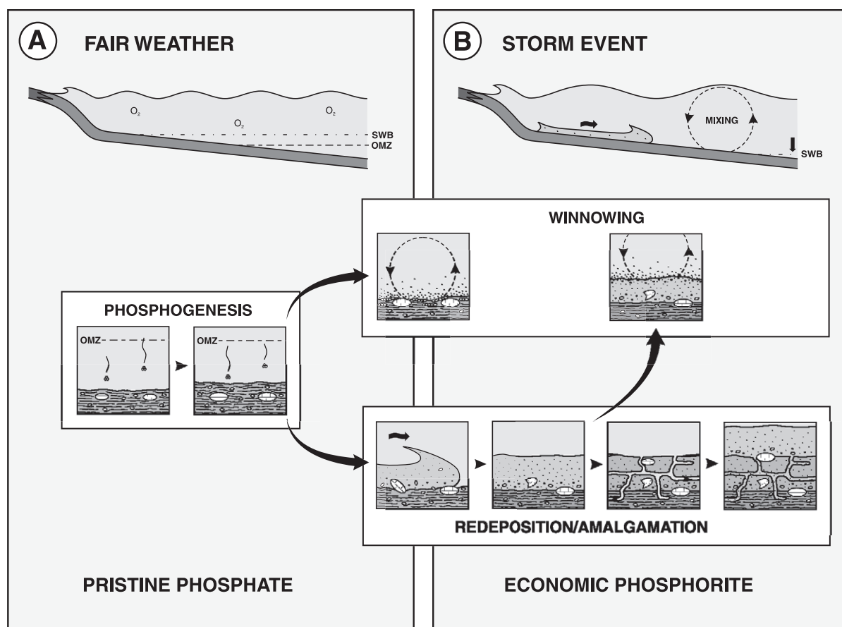
Fig. 8. Depositional model for the formation of economic phosphorite. (A) Pristine phosphate forms during “fairweather” periods under a stratified water column with a well developed oxygen minimum (OMZ) and a shallow storm-wave base (SWB). Phosphogenesis is stimulated by high surface productivity and relative stratigraphic condensation. (B) With an increase in storm frequency and intensity with time, the SWB deepens and destratifies the water column. Economic phosphorites form through the amalgamation of storm-induced event beds derived from pristine phosphate facies. Both pristine phosphate facies and the tops of economic phosphorite beds may undergo storm wave winnowing during storm events.
