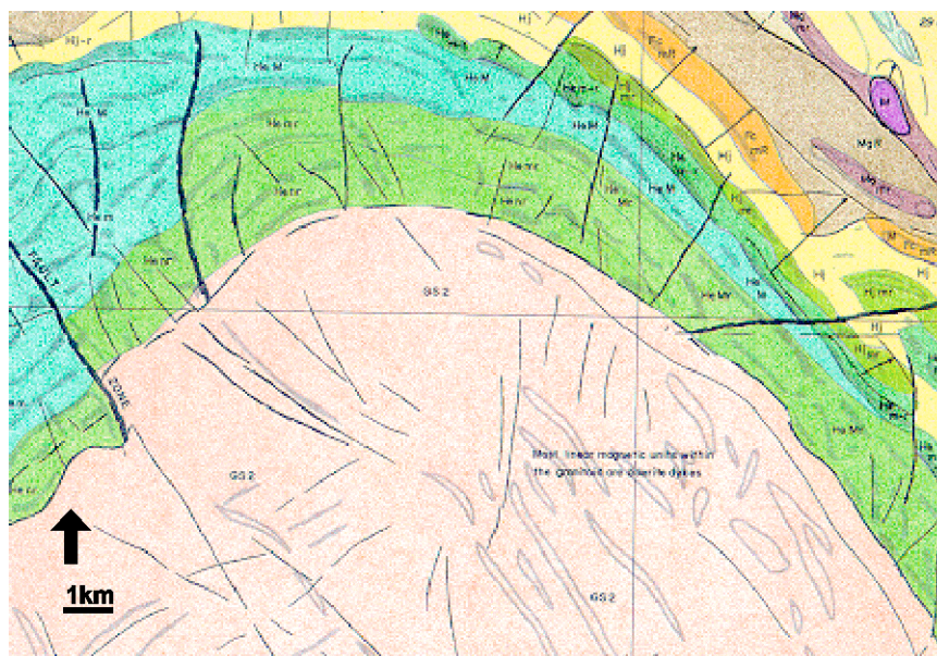
Figure 7: An extract from the southern part of the Kennedy Gap 1:100 000 scale geomagnetic / radiometric interpretation map.
