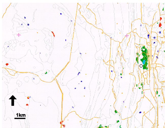
Figure 12: An extract from the Mount Isa 1:100 000 scale radiometric depletion map. The lithological boundaries are in grey, roads in gold and the ternary image (K:Th:U = R:G:B) highlights areas of K, Th and U depletion.
