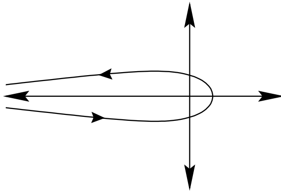
Figure 35.1: The Hankel Contour.
