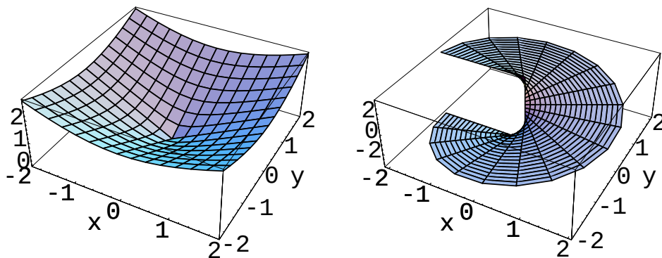
Figure 9.6: A Few Branches of \arg(z)
