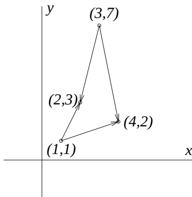
Figure 4.15: Quadrilateral
