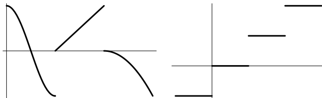
Figure 5.4: Piecewise Continuous Functions
