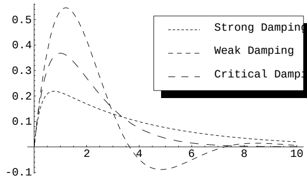
Figure 19.4: Strongly, weakly and critically damped solutions.
