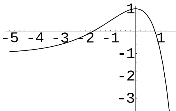
Figure 16.6: The function 2(1-x)e^x - 1 .
