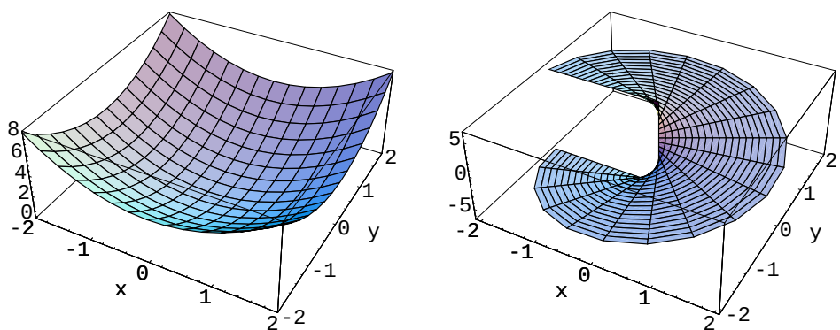
Figure 9.9: Plots of |z^2| and a branch of \arg(z^2)
