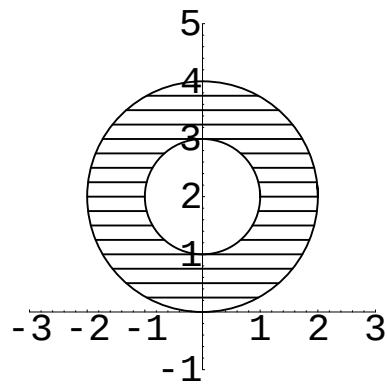
Figure 8.13: 1 < |z - 2i| < 2
