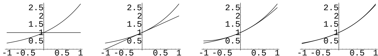
Figure 5.11: Four Finite Taylor Series Approximations of e^x
