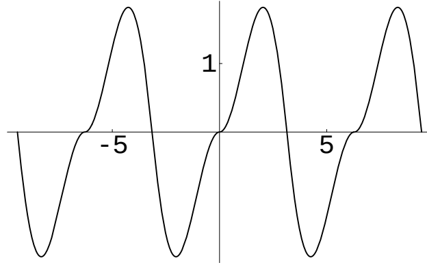
Figure 30.12: The odd periodic extension of x \sin x .
