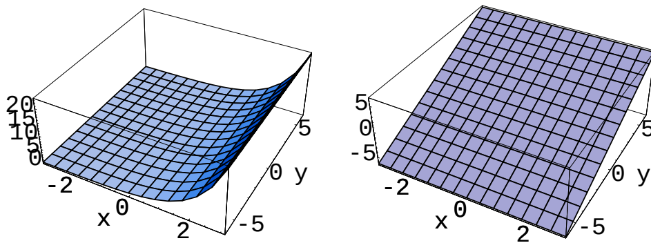
Figure 9.11: Plots of |e^z| and a branch of \arg(e^z)
