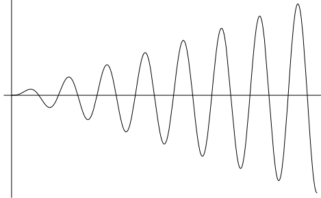
Figure 23.6: Resonant Forcing
