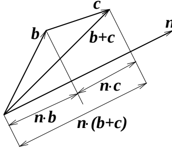
Figure 4.12: The Distributive Law for the Dot Product
