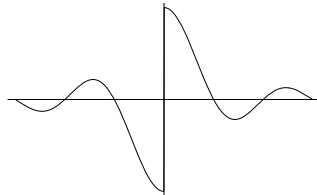
Figure 5.2: Plot of \sin(x)/|x| .
