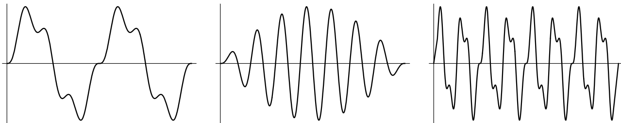
Figure 23.5: Non-resonant Forcing
