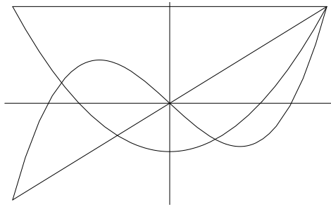
Figure 25.4: The First Four Legendre Polynomials
