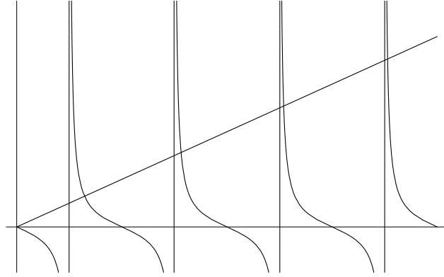
Figure 31.1: x and -\tan(x) .
