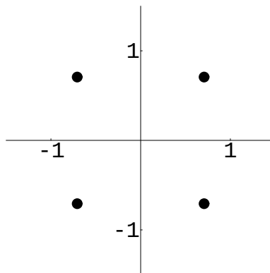
Figure 8.9: (-1)^{-3/4}
