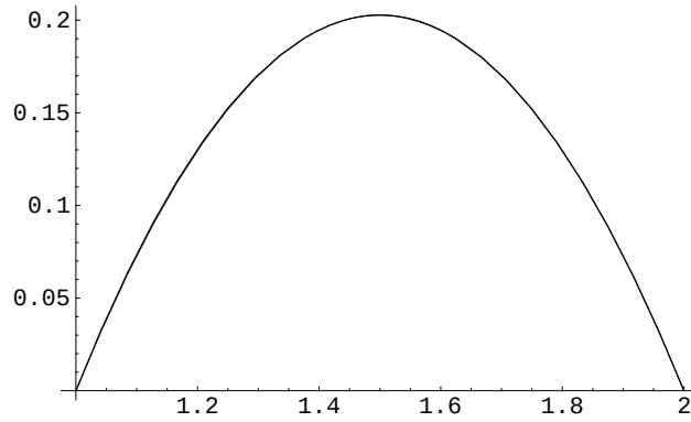
Figure 49.11: One Term Polynomial Approximation and Exact Solution.
