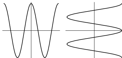
Figure 3.8: y = \cos x and y = \arccos x
