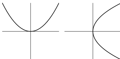
Figure 3.2: Diagrams of One-To-One, Many-To-One and One-To-Many Functions
