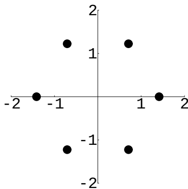
Figure 8.10: 8^{1/6}
