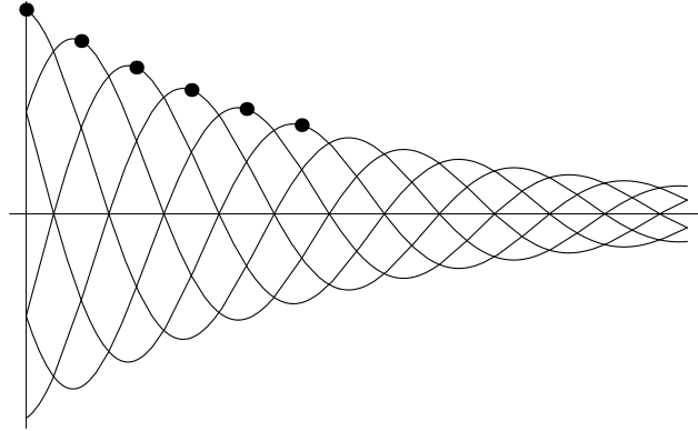
Figure 41.3: An Exponentially Decaying, Traveling Wave
