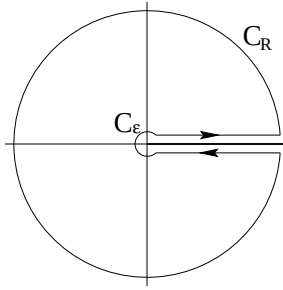
Figure 15.6:
