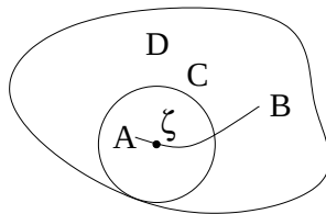
Figure 11.3: Domain Containing Arc Along Which f(z) Vanishes
