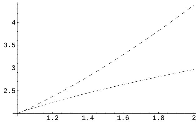
Figure 49.1:
