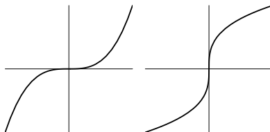
Figure 3.7: y = x^3 and y = x^{1/3}
