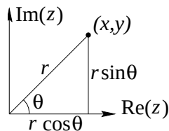
Figure 8.4: Polar Form
