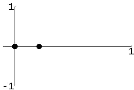
Figure 9.31: (-i)^{-i}
