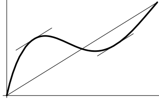
Figure 5.10: Theorem of the Mean.
