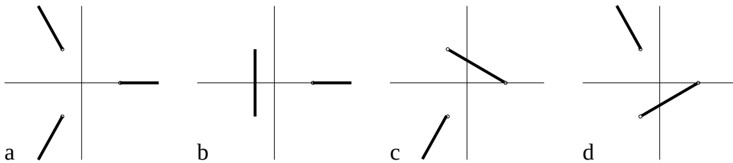
Figure 9.36: (z^3 - 1)^{1/2}
