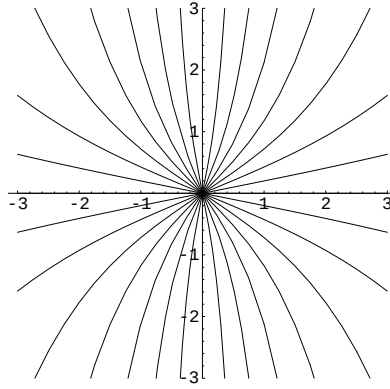
Figure 49.4: \sinh(cx)
