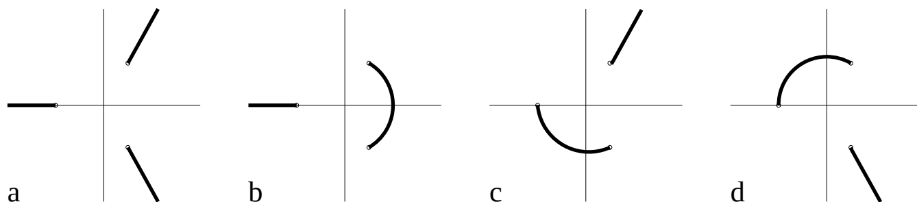
Figure 9.38: (z^3 + 8)^{1/2}
