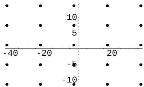
Figure 9.35: \log((1+i)^{i\pi})
