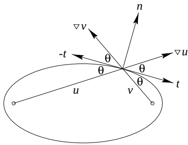
Figure 7.3: An ellipse and rays from the foci.
