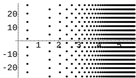
Figure 9.33: \log(\log(i))
