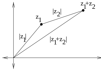
Figure 8.8: Triangle Inequality
