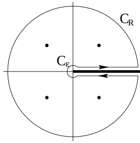
Figure 15.11: Possible Path of Integration for f(z) = \frac{z^a}{1+z^4}
