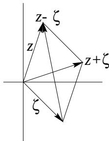
Figure 8.18: The parallelogram defined by z and \zeta .
