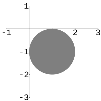
Figure 8.15: |z - 1 + i| < 1
