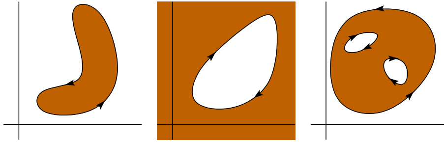
Figure 9.3: Traversing the boundary in the positive direction.
