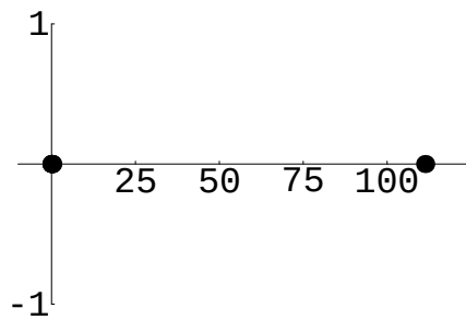
Figure 9.34: i^i
